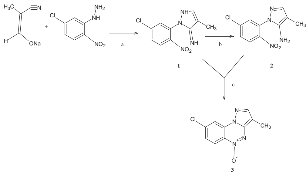
Scheme 1. Reagents and conditions: (a) Ethanol /HCl, 80 °C 2 h; (b) Ethanol /HCl, 80 °C 10 h; (c) NaOH 10%, 50 °C.
